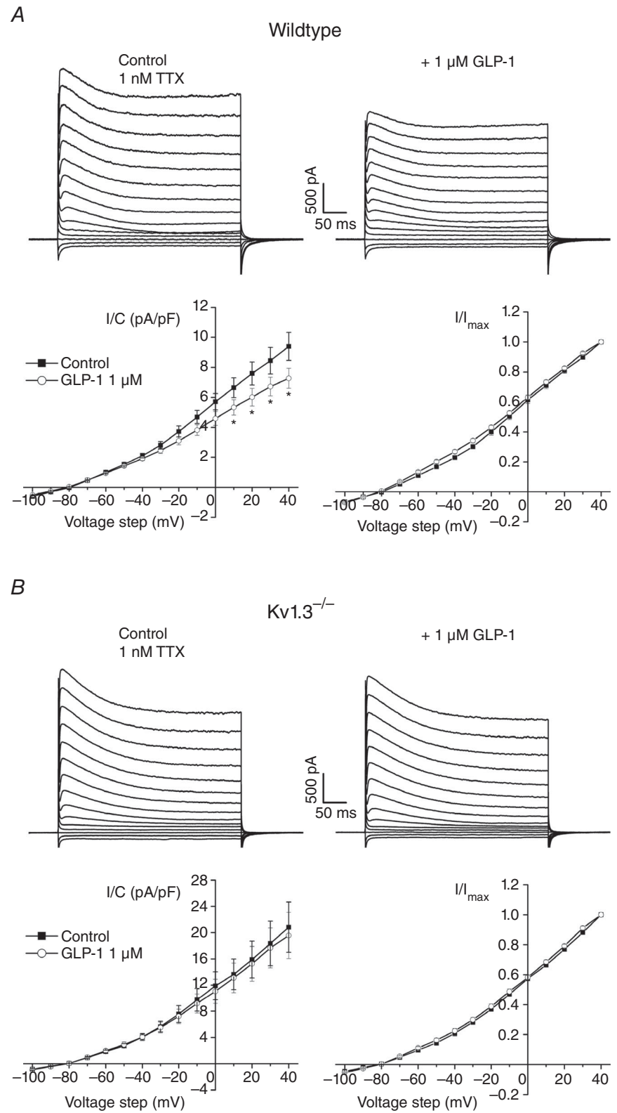
Figure 9. The magnitude of MC voltage-activated outward currents are decreased following GLP-1 application in WT mice but not for mice with a Kv1.3-targeted deletion (Kv1.3 -/- )
